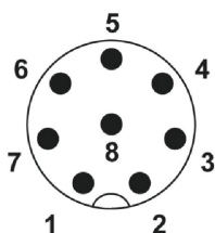
M12 male connector
