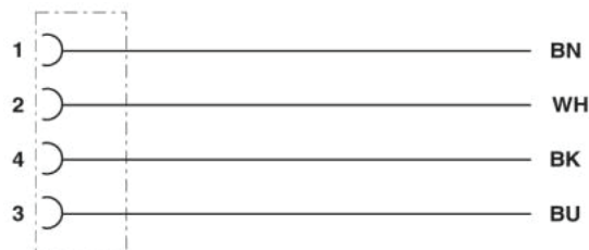
Flexible wires
