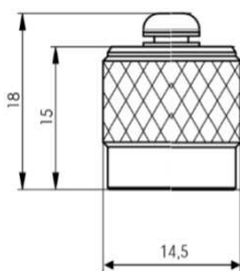
3x TNCrev Protective cap Antenna Port
