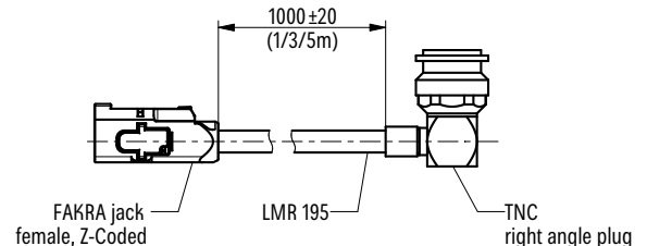
Connecting Cable 52010461/52010462/52010463
