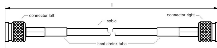
Connecting Cable 52010174/52010175/52010176/52010177
