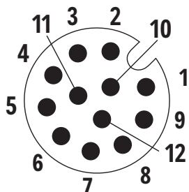
Schematic Diagram - M12, 12-pin, A-coded, male
