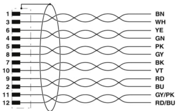
Circuit Diagram - Allocation of the M12 plug
